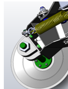
FIGURE 24 - DISC SCALPER ATTACHMENT.
