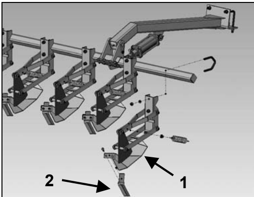
FIGURE 22 - KNIFE SCALPER ADJUSTMENT
