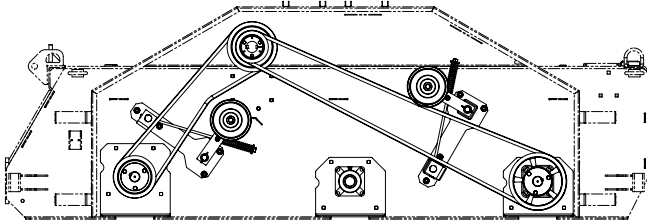
FIGURE 21 - LH DRIVES, STEEL FLAILS.
