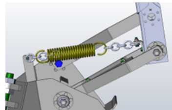
FIGURE 23_1 - DISC SCALPER SPRING.
