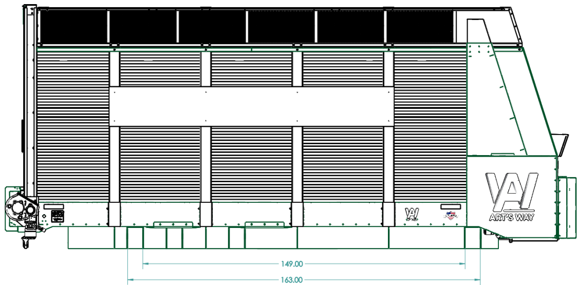
18' BOX SPACING 1
