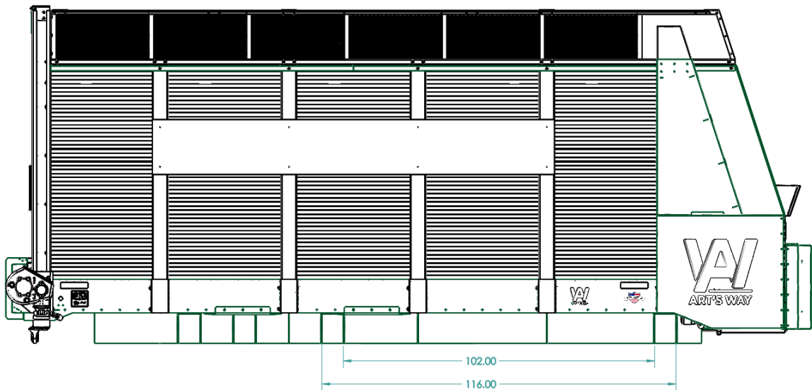
18' BOX SPACING 3
